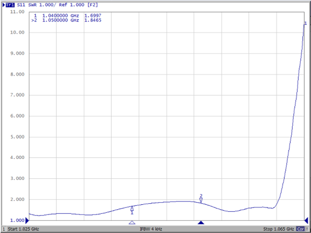
S11
