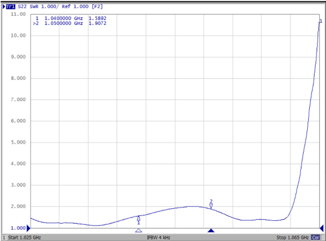
S22
